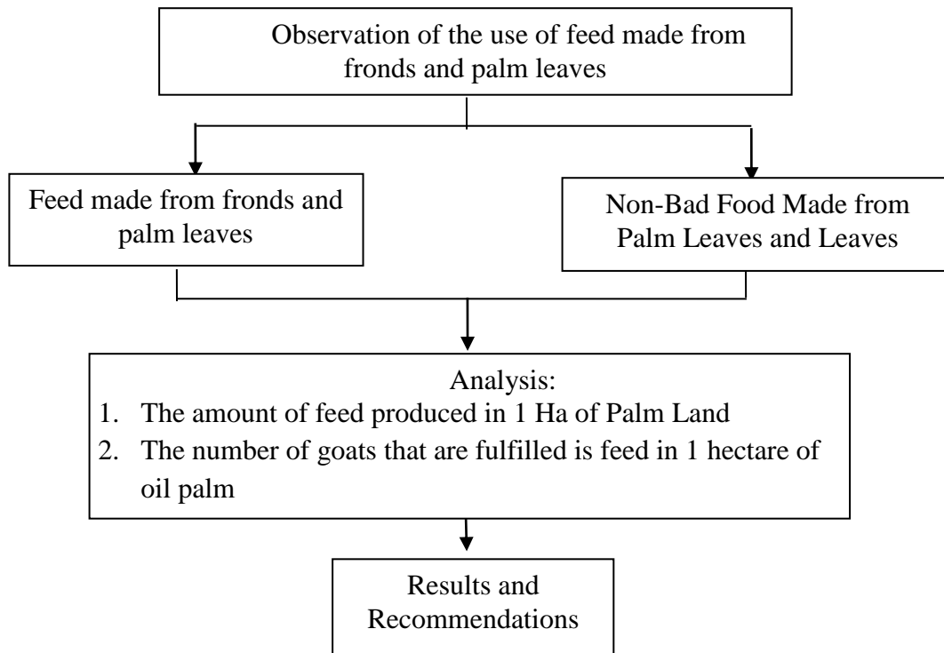
Figure 1. Research Flowchart
